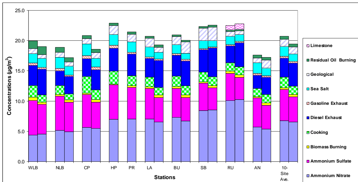
Figure VII-12. First & Second-Year PM 2.5 Source Contribution Comparison Basin Gasoline Profile
