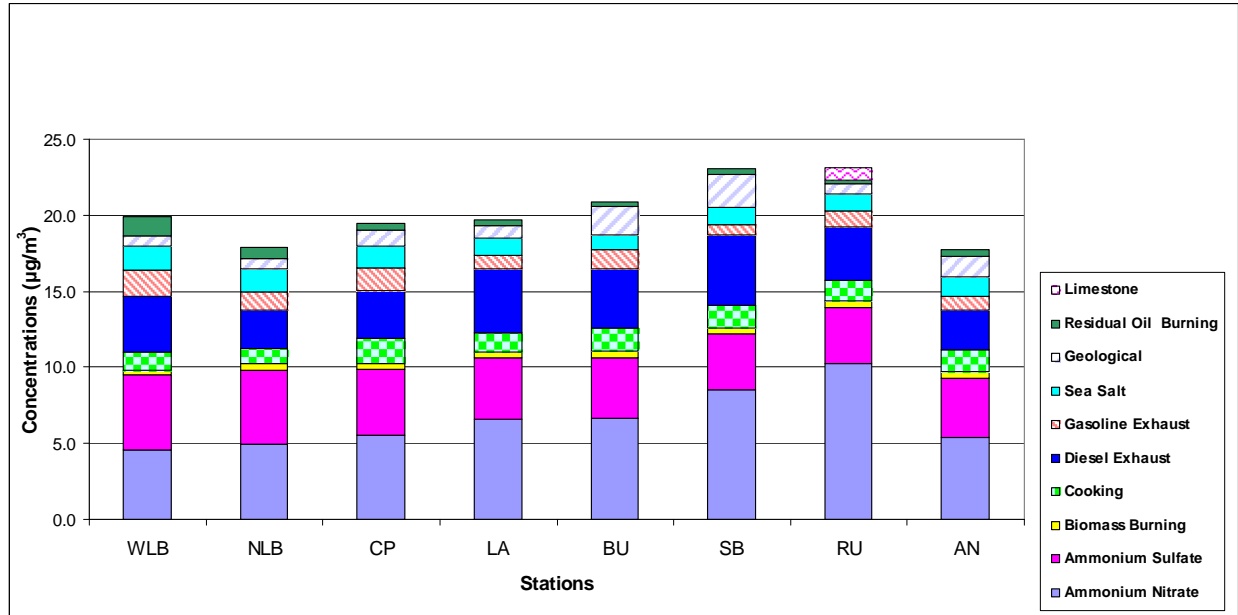
Figure VII-10. Second-Year PM 2.5 Source Contribution Estimates – NFRAQS Gasline Profile
