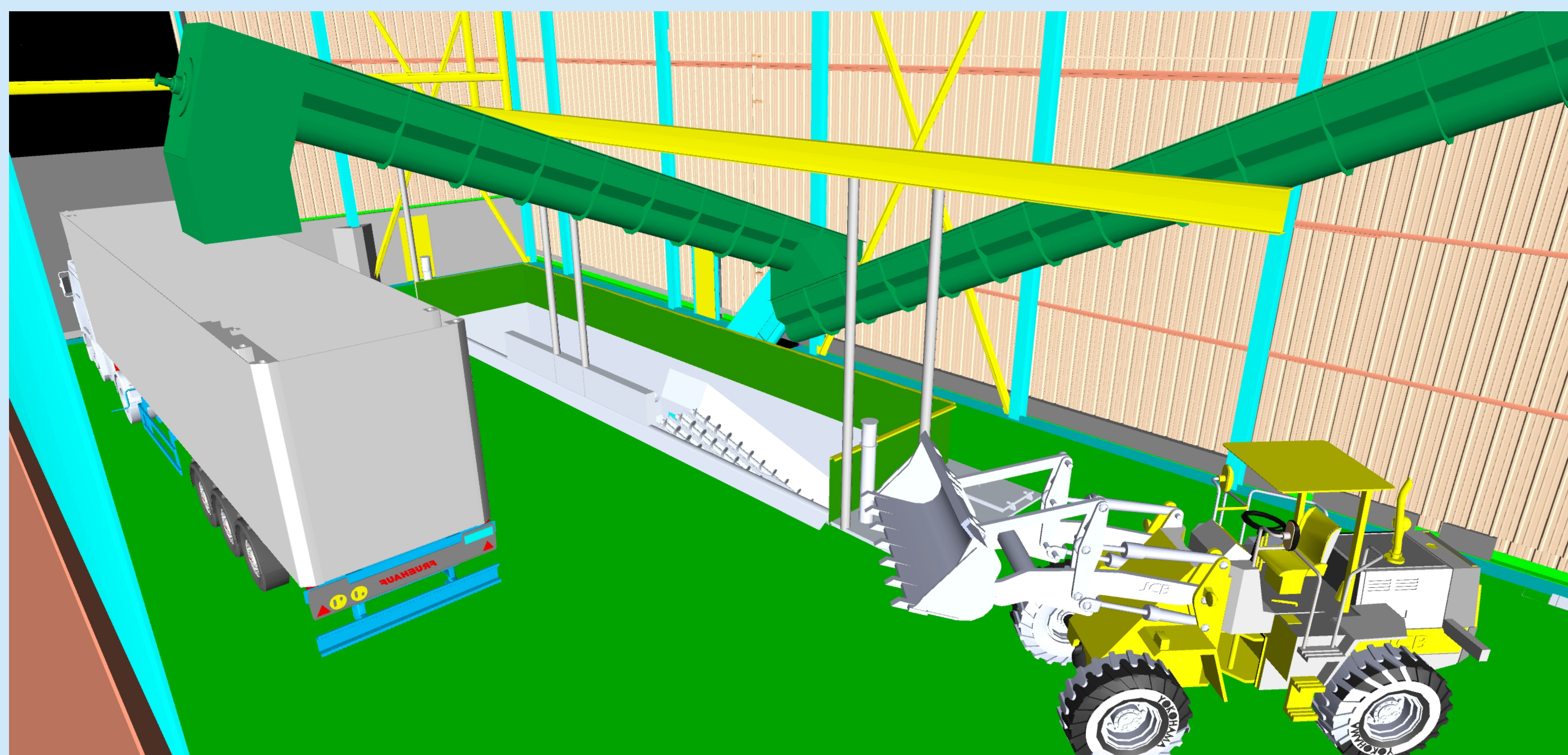
Rendering of Permanent Total Enclosure
