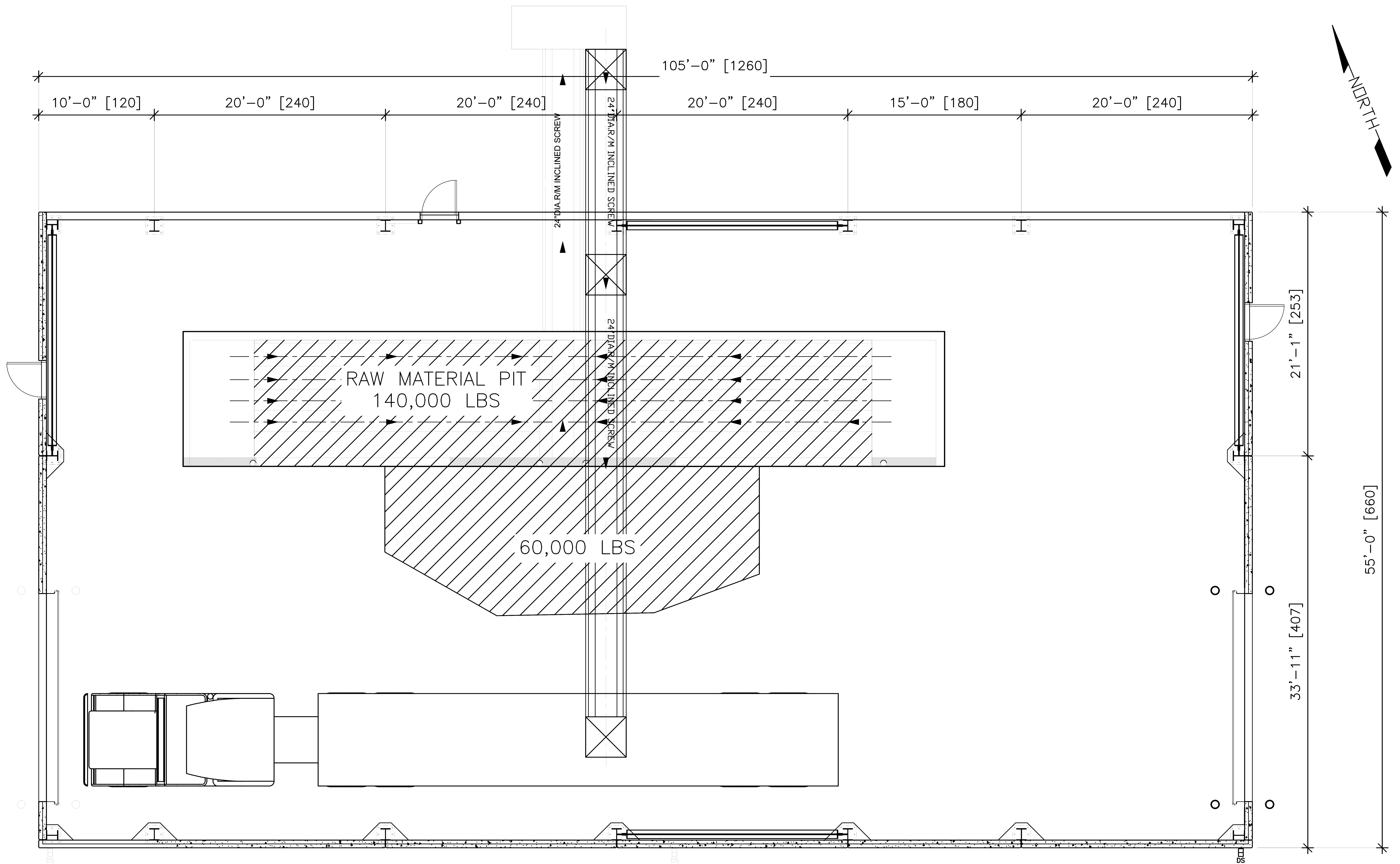
R/M PIT ENCLOSURE
